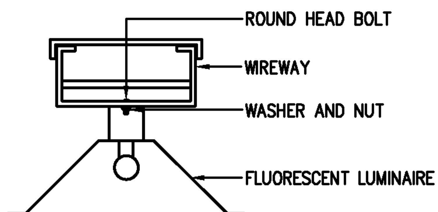
SECTION A
