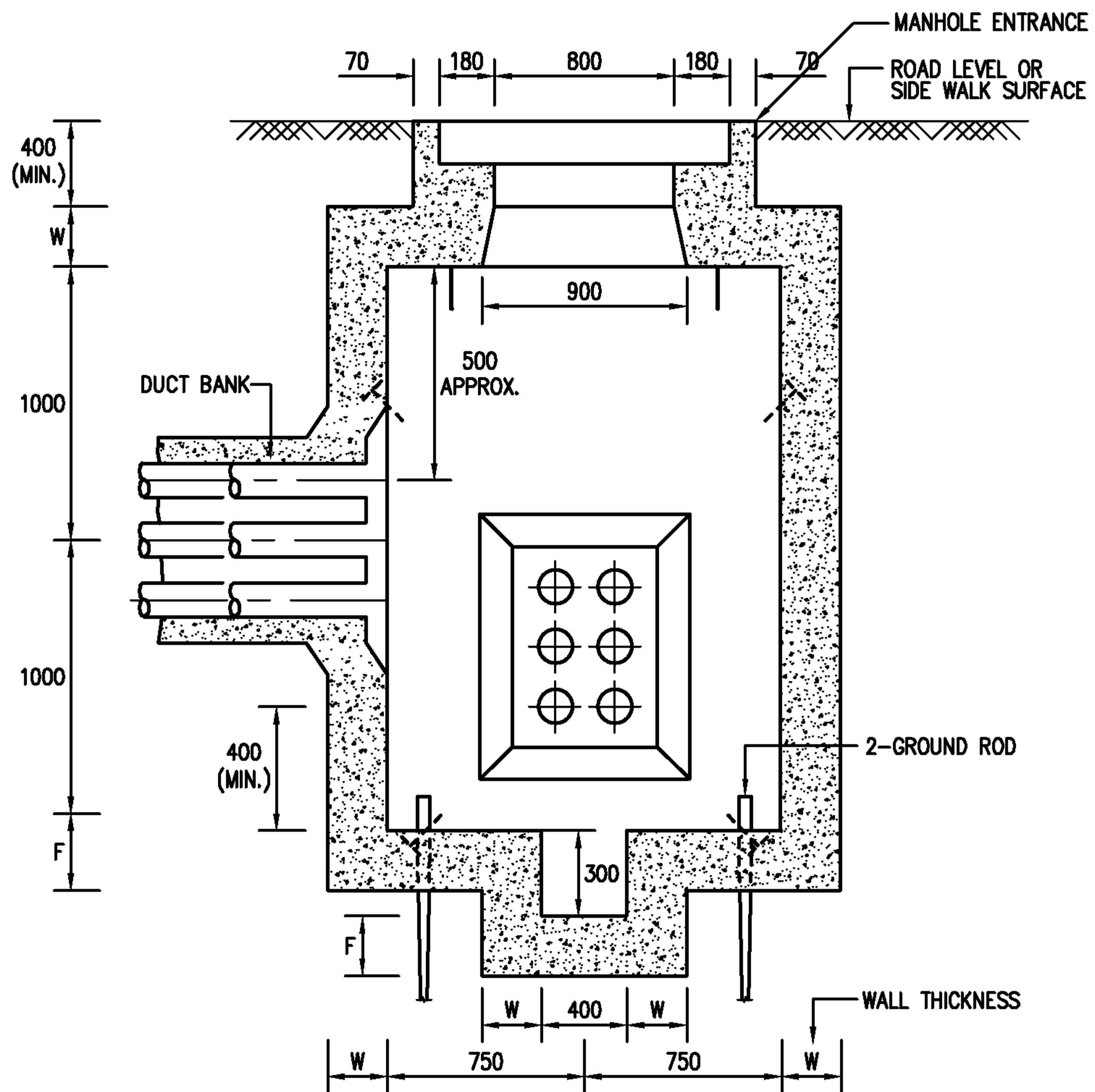
SECTION B
