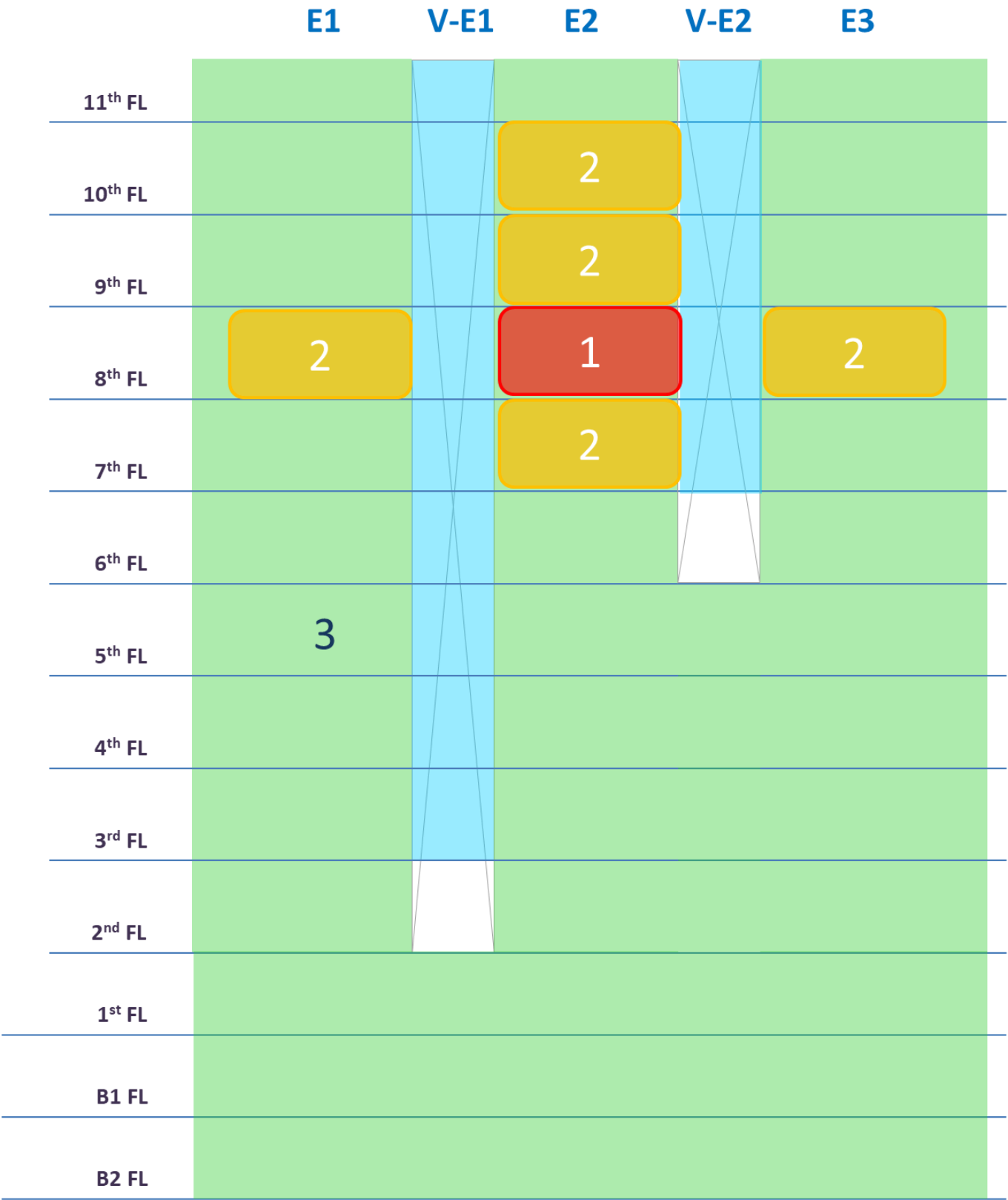
East - Zone Fire Alarm Sequence
