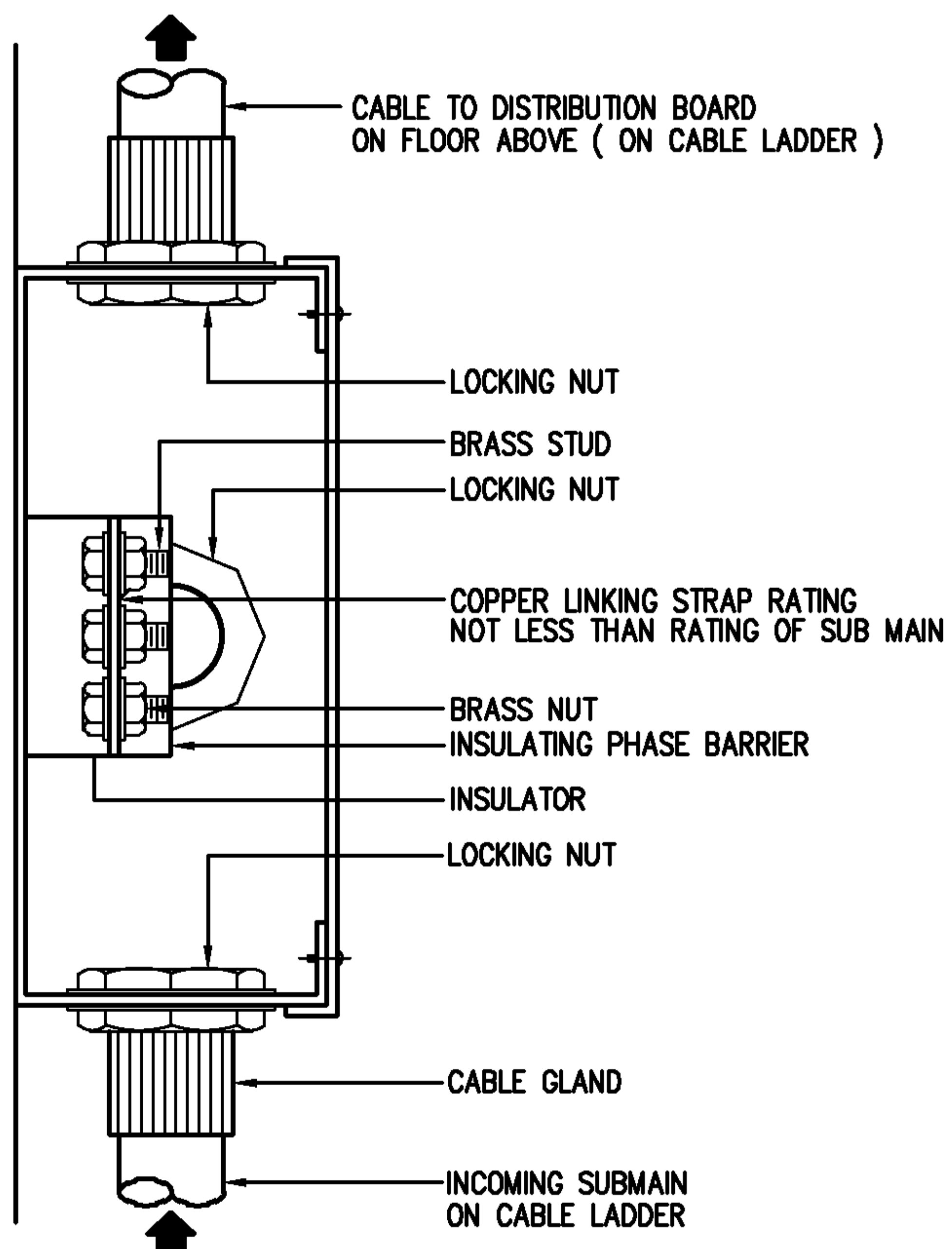
SECTION A
